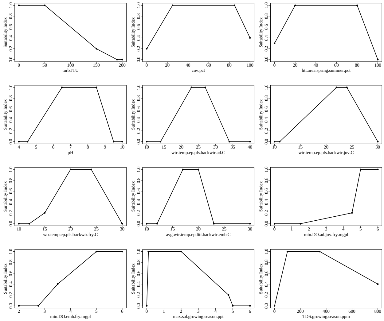
Figure 1. Suitability index graphs for variables included in the blackcrappieLacSal model in ecoREST.
